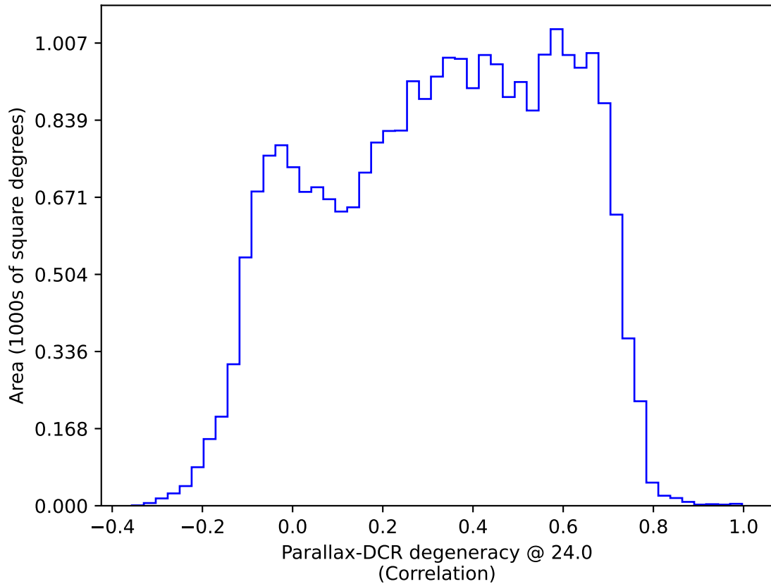
too_elab_heavy_r64_d3_gz_v3.4_10yrs All sky: Parallax-DCR degeneracy @ 24.0
