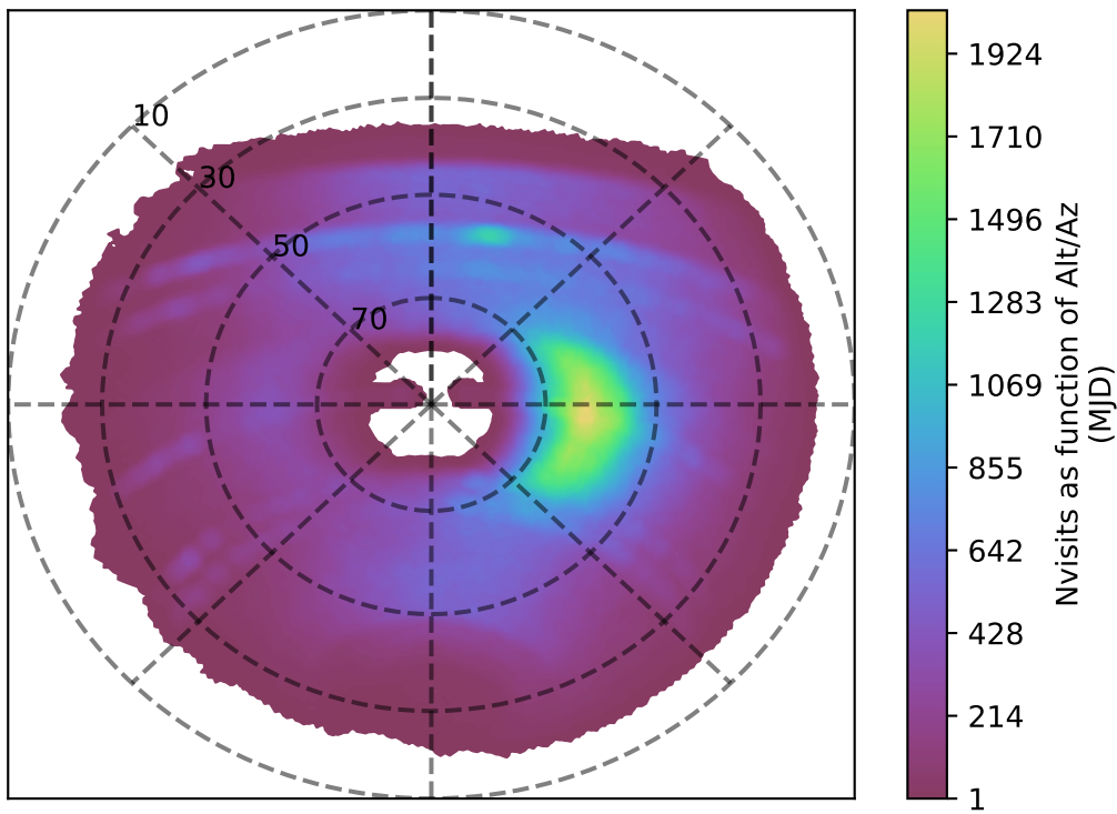
too_elab_heavy_r64_d3_gz_v3.4_10yrs y band: Nvisits as function of Alt/Az
