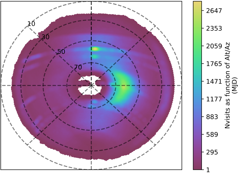
too_elab_heavy_r64_d3_gz_v3.4_10yrs i band: Nvisits as function of Alt/Az
