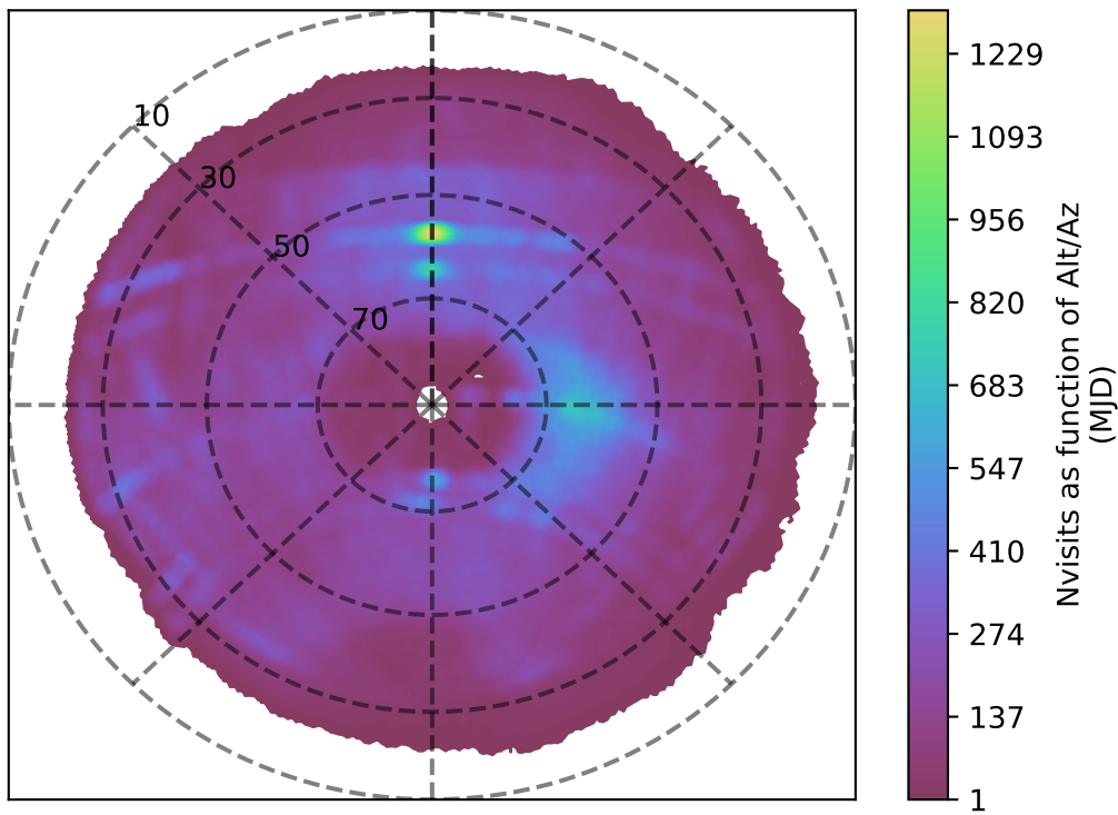
too_elab_heavy_r64_d3_gz_v3.4_10yrs g band: Nvisits as function of Alt/Az
