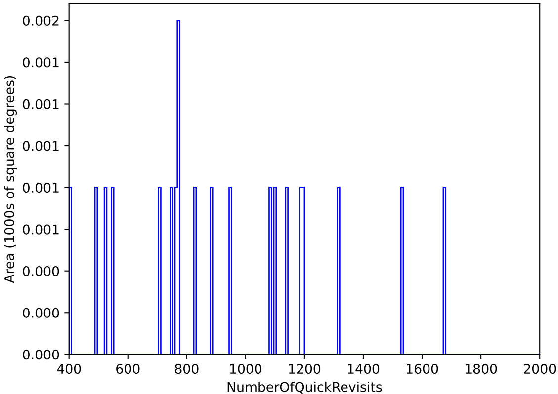
too_elab_heavy_r64_d3_gz_v3.4_10yrs WFD: NumberOfQuickRevisits
