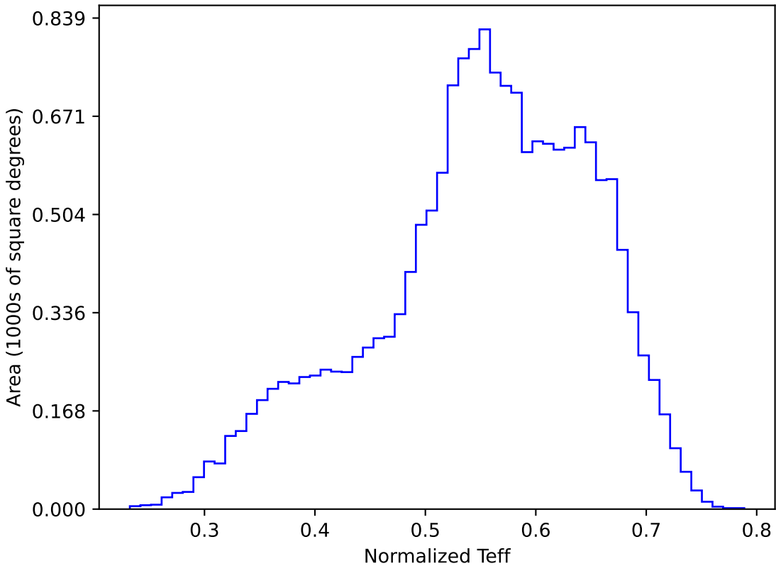
too_elab_heavy_r64_d3_gz_v3.4_10yrs WFD y band: Normalized Teff
