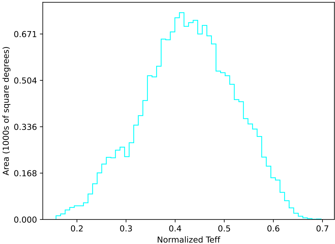
too_elab_heavy_r64_d3_gz_v3.4_10yrs WFD u band: Normalized Teff
