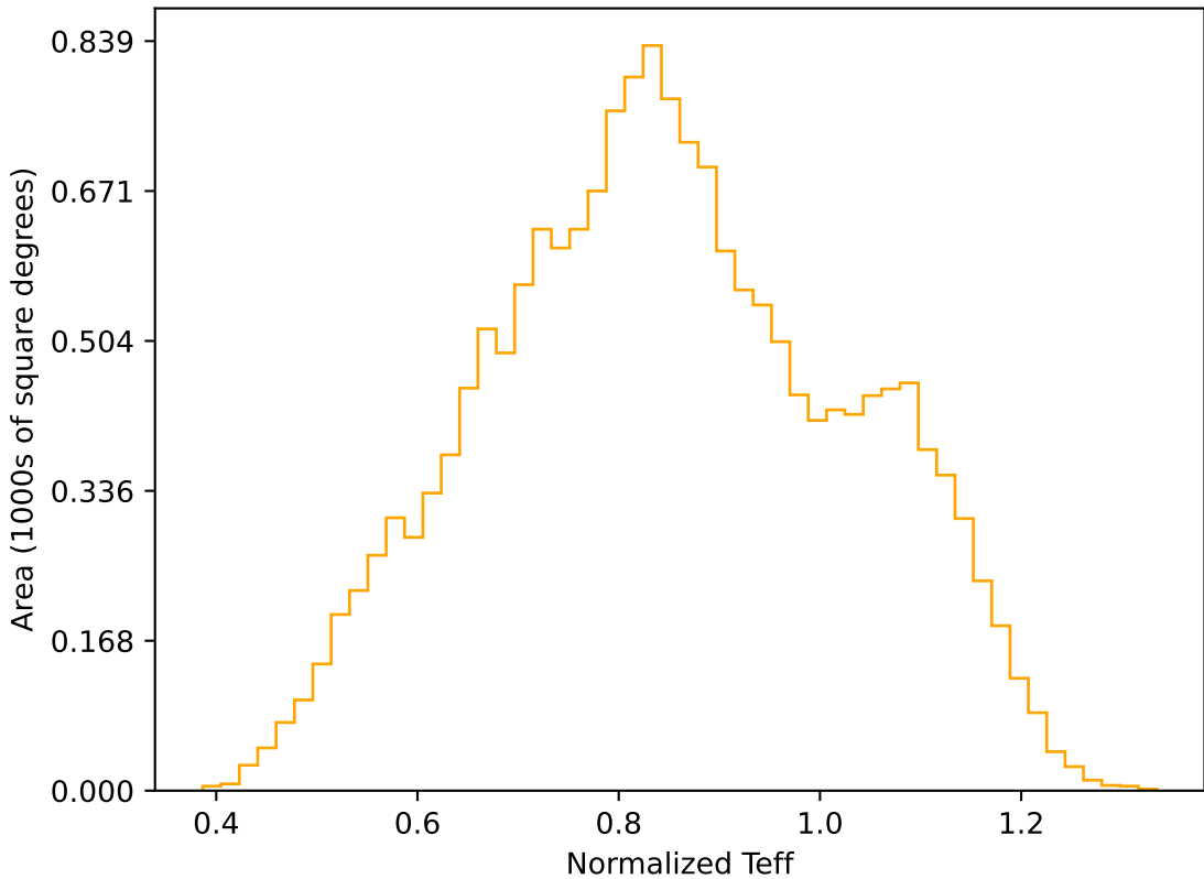
too_elab_heavy_r64_d3_gz_v3.4_10yrs WFD r band: Normalized Teff
