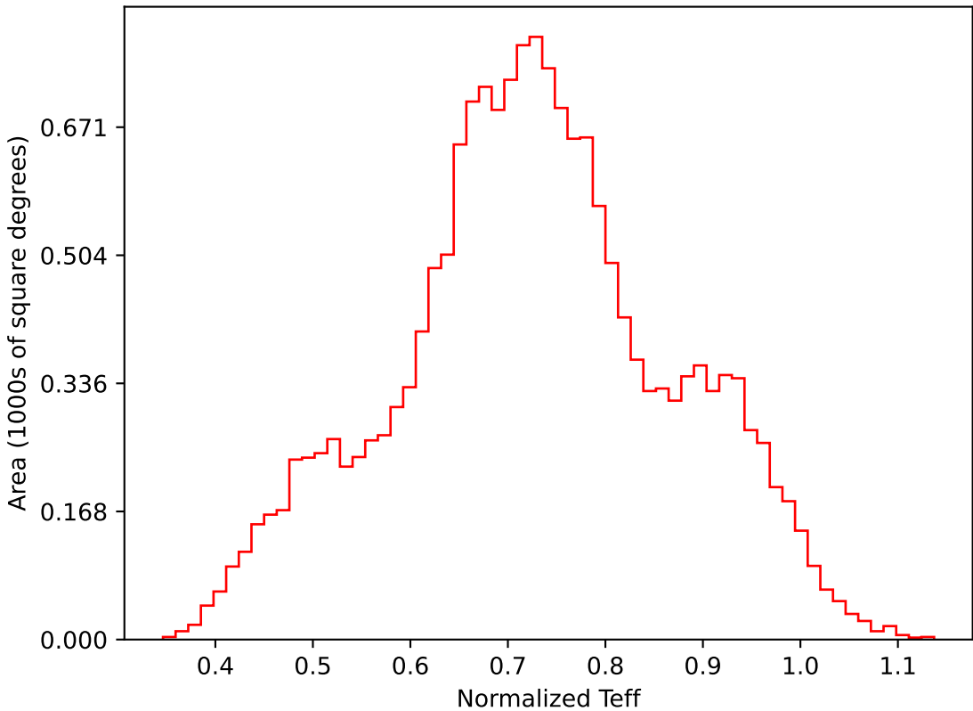
too_elab_heavy_r64_d3_gz_v3.4_10yrs WFD i band: Normalized Teff
