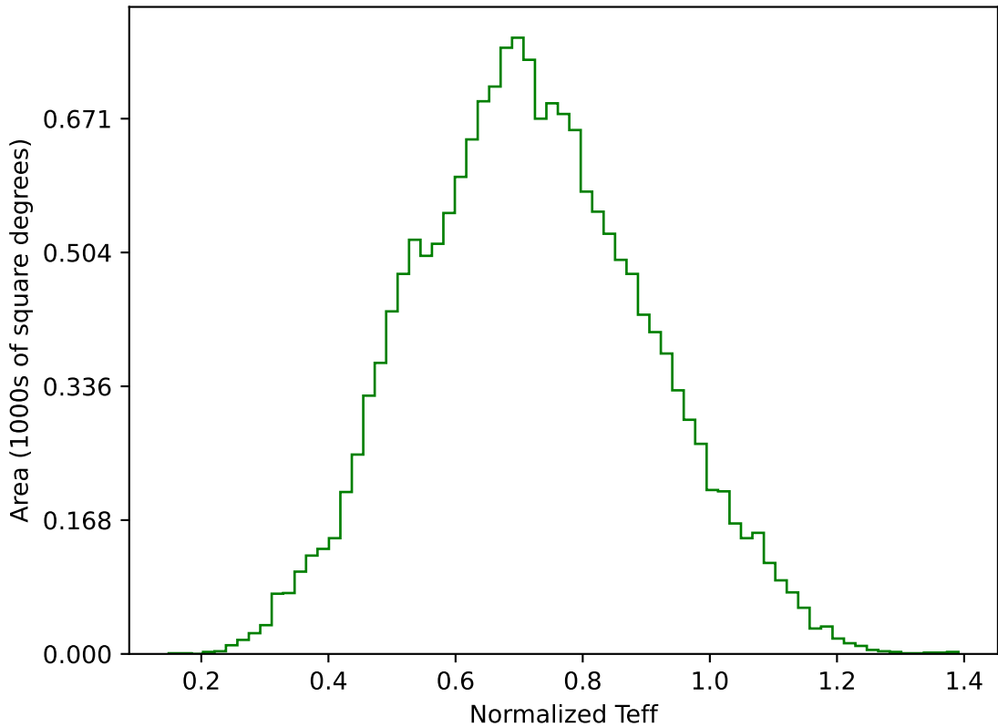
too_elab_heavy_r64_d3_gz_v3.4_10yrs WFD g band: Normalized Teff
