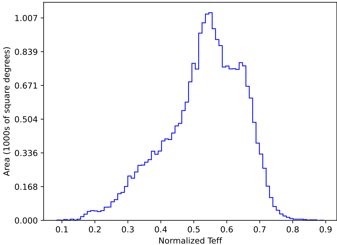
too_elab_heavy_r64_d3_gz_v3.4_10yrs All sky y band: Normalized Teff
