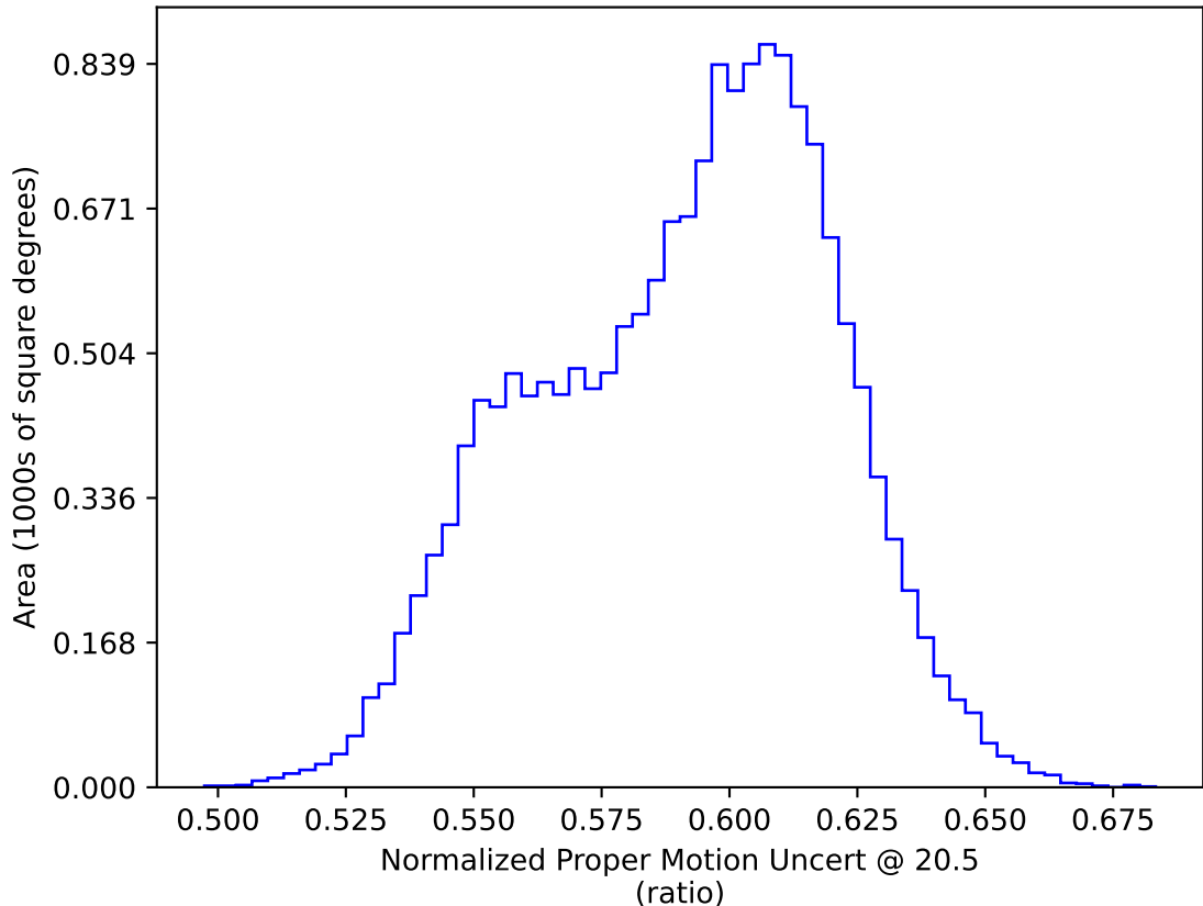
too_elab_heavy_r64_d3_gz_v3.4_10yrs WFD: Normalized Proper Motion Uncert @ 20.5
