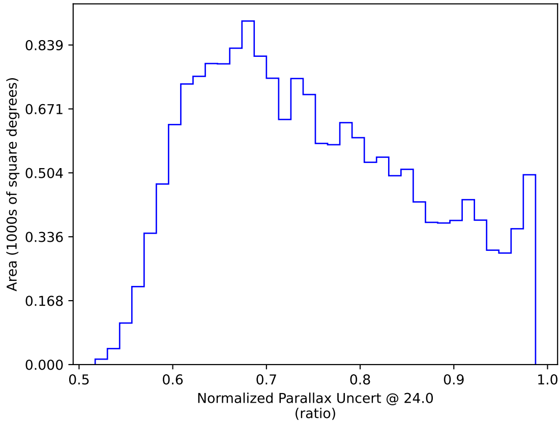
too_elab_heavy_r64_d3_gz_v3.4_10yrs WFD: Normalized Parallax Uncert @ 24.0
