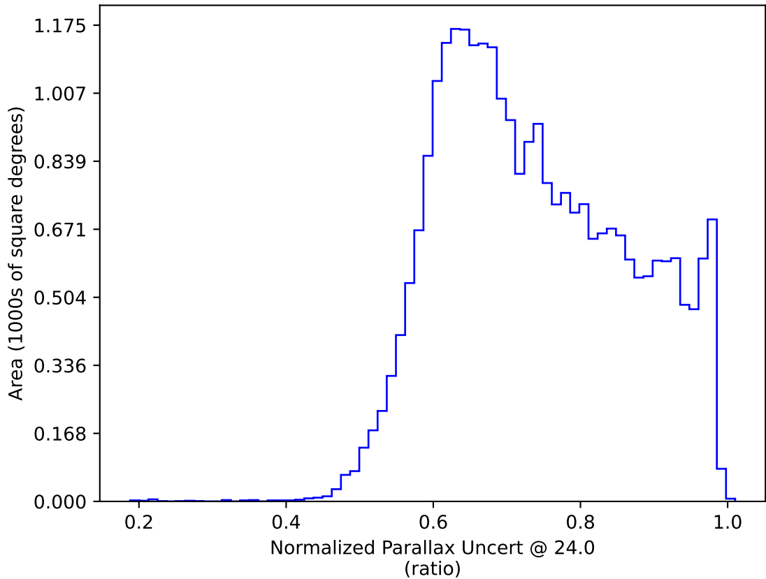
too_elab_heavy_r64_d3_gz_v3.4_10yrs All sky: Normalized Parallax Uncert @ 24.0
