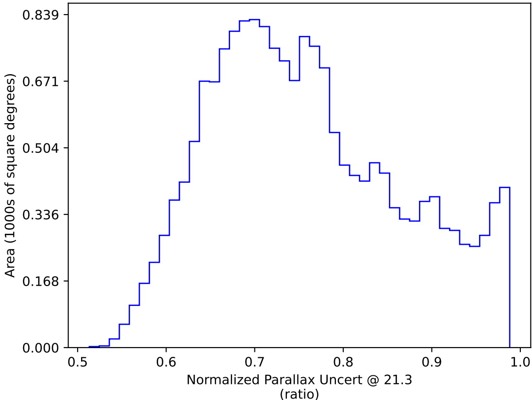
too_elab_heavy_r64_d3_gz_v3.4_10yrs WFD y band only: Normalized Parallax Uncert @ 21.3
