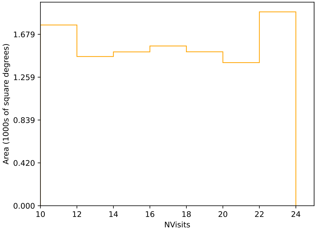
too_elab_heavy_r64_d3_gz_v3.4_10yrs Yr 3-4 r band: NVisits
