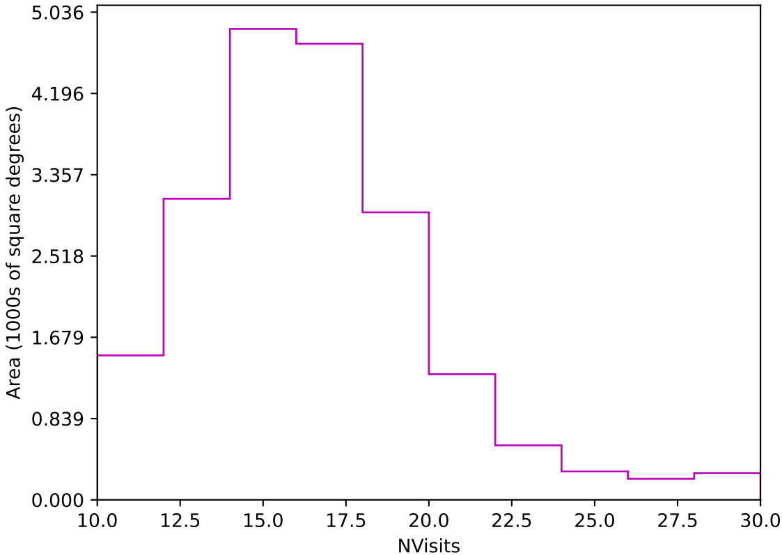
too_elab_heavy_r64_d3_gz_v3.4_10yrs Yr 1 z band: NVisits
