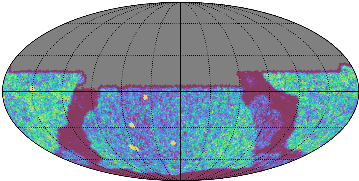
too_elab_heavy_r64_d3_gz_v3.4_10yrs Yr 1 y band: NVisits
