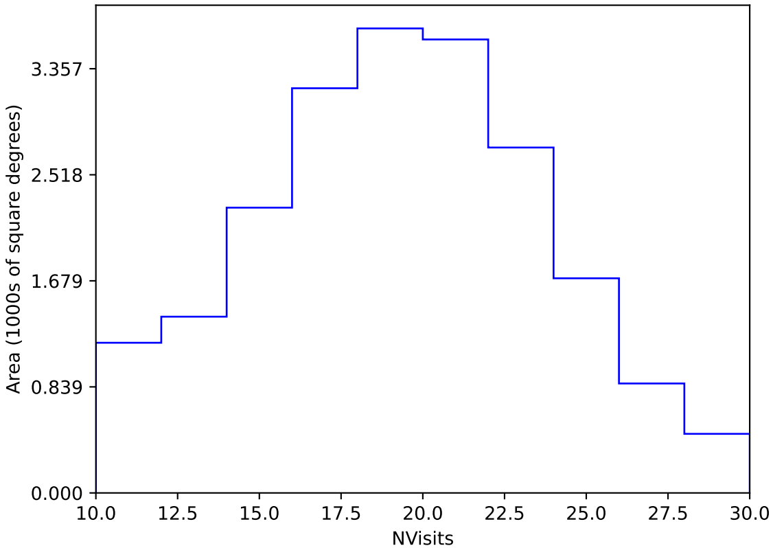
too_elab_heavy_r64_d3_gz_v3.4_10yrs Yr 1 y band: NVisits
