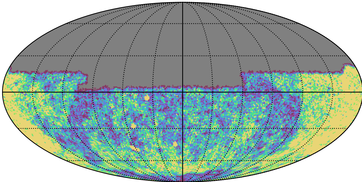
too_elab_heavy_r64_d3_gz_v3.4_10yrs Yr 1 u band: NVisits
