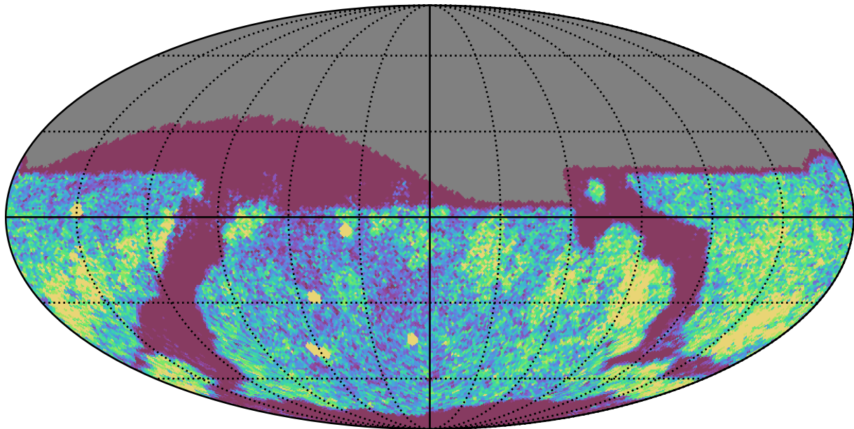
too_elab_heavy_r64_d3_gz_v3.4_10yrs Yr 1 r band: NVisits
