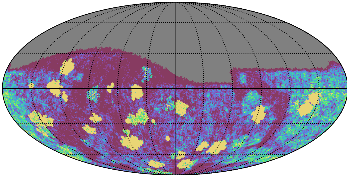
too_elab_heavy_r64_d3_gz_v3.4_10yrs Yr 1 g band: NVisits
