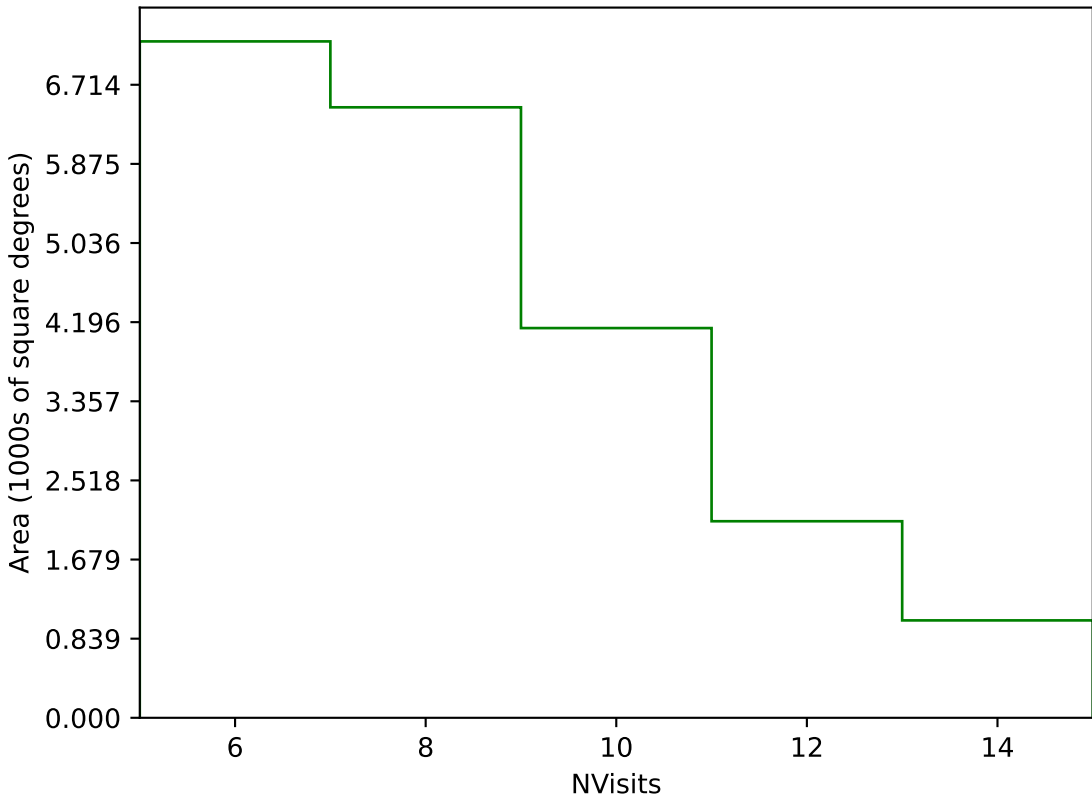
too_elab_heavy_r64_d3_gz_v3.4_10yrs Yr 1 g band: NVisits
