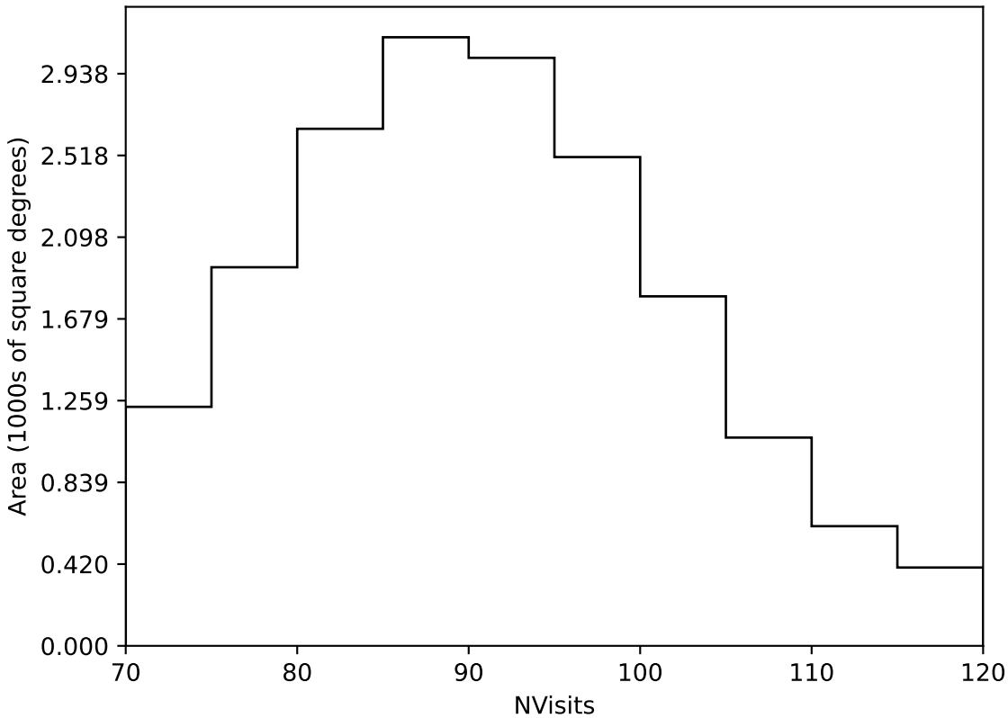
too_elab_heavy_r64_d3_gz_v3.4_10yrs Yr 1 all bands: NVisits
