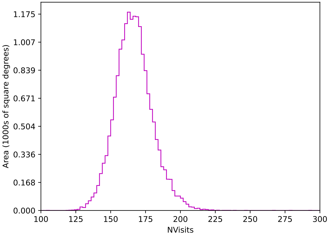
too_elab_heavy_r64_d3_gz_v3.4_10yrs WFD z band: NVisits
