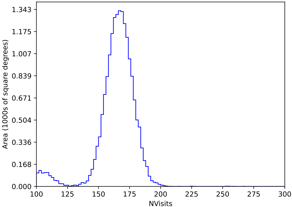
too_elab_heavy_r64_d3_gz_v3.4_10yrs WFD y band: NVisits
