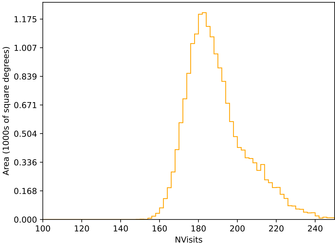
too_elab_heavy_r64_d3_gz_v3.4_10yrs WFD r band: NVisits
