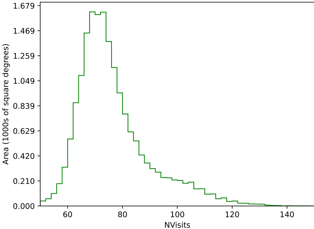
too_elab_heavy_r64_d3_gz_v3.4_10yrs WFD g band: NVisits
