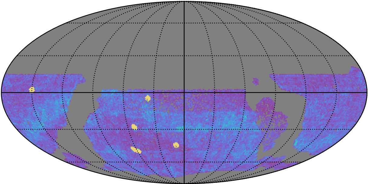
too_elab_heavy_r64_d3_gz_v3.4_10yrs WFD all bands: NVisits
