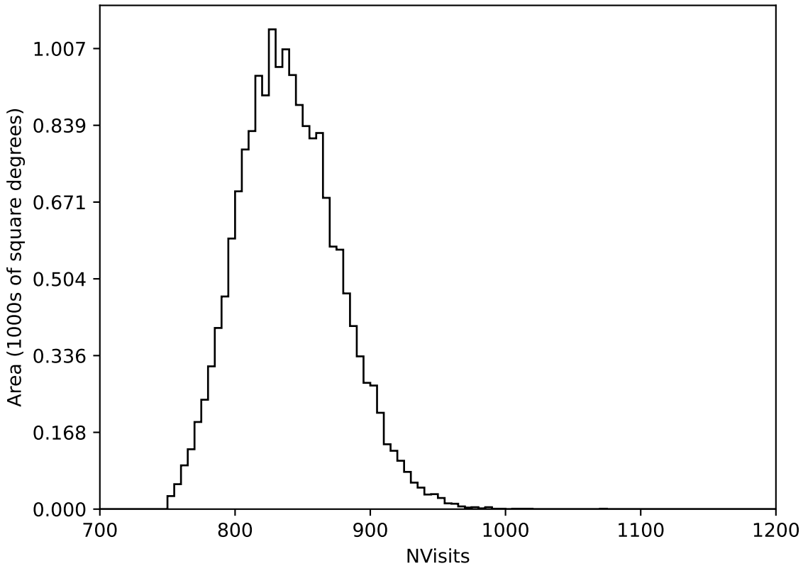
too_elab_heavy_r64_d3_gz_v3.4_10yrs WFD all bands: NVisits
