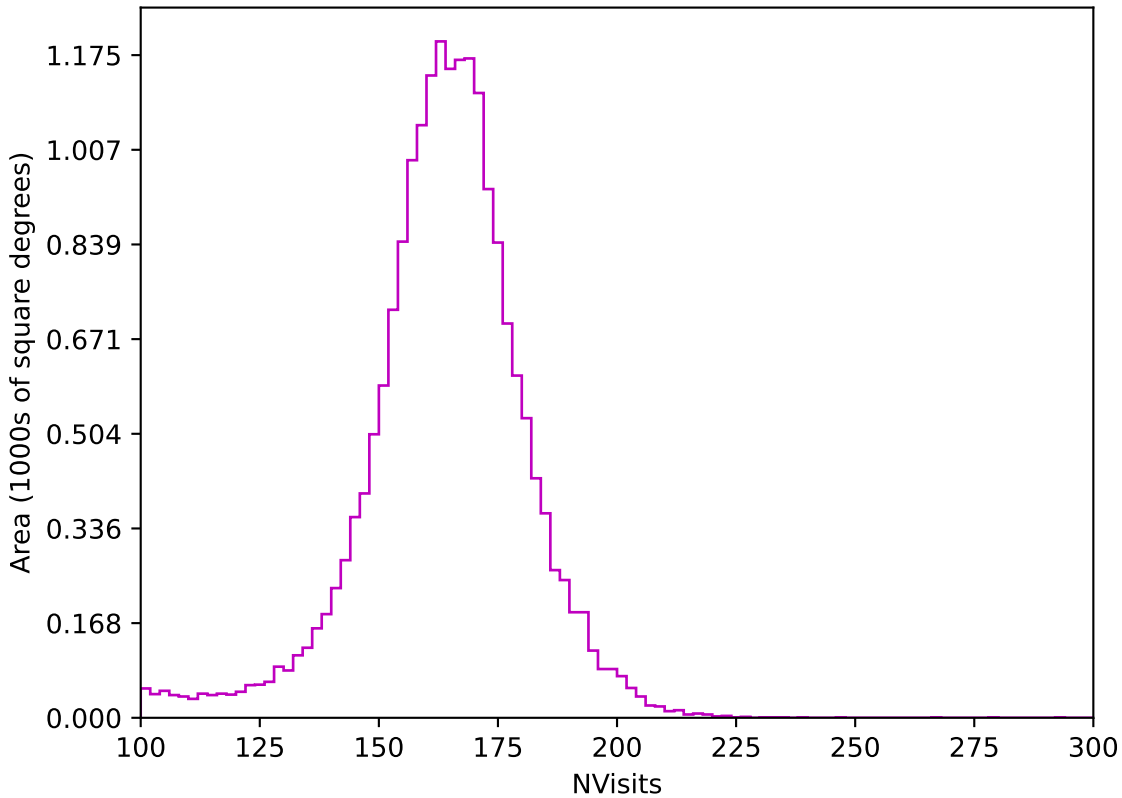
too_elab_heavy_r64_d3_gz_v3.4_10yrs All sky z band: NVisits
