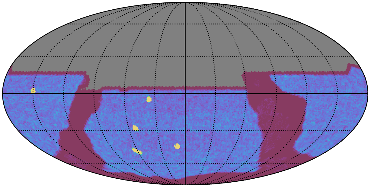
too_elab_heavy_r64_d3_gz_v3.4_10yrs All sky y band: NVisits
