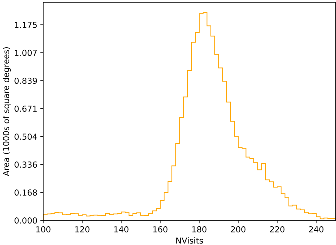
too_elab_heavy_r64_d3_gz_v3.4_10yrs All sky r band: NVisits
