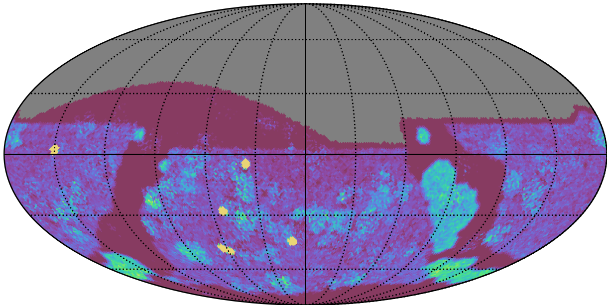
too_elab_heavy_r64_d3_gz_v3.4_10yrs All sky g band: NVisits
