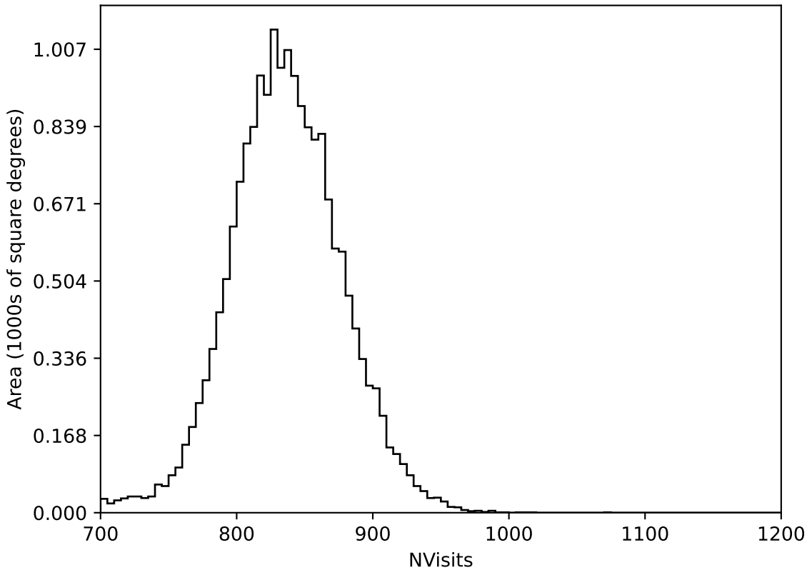
too_elab_heavy_r64_d3_gz_v3.4_10yrs All sky all bands: NVisits
