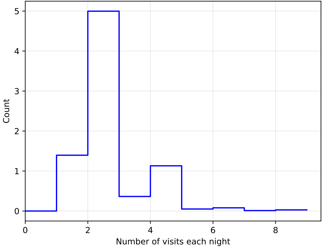
too_elab_heavy_r64_d3_gz_v3.4_10yrs WFD: NVisitsPerNight 1e6
