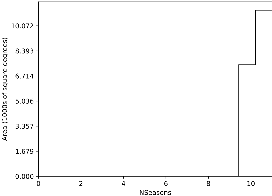
too_elab_heavy_r64_d3_gz_v3.4_10yrs WFD all bands: NSeasons
