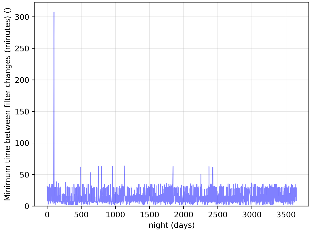
too_elab_heavy_r64_d3_gz_v3.4_10yrs Per Night: Minimum time between filter changes (minutes)
