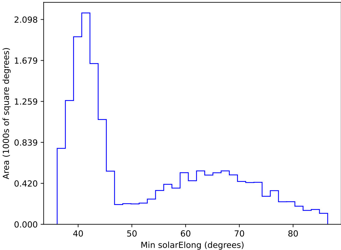
too_elab_heavy_r64_d3_gz_v3.4_10yrs WFD z band: Min solarElong
