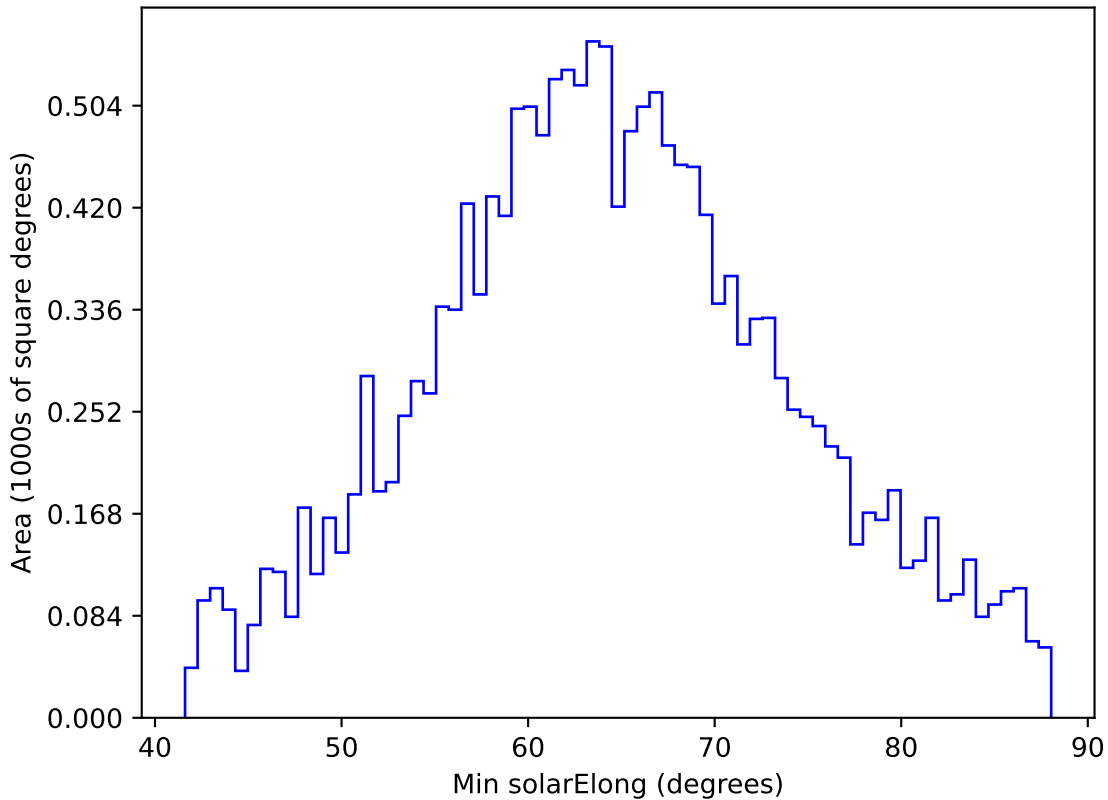
too_elab_heavy_r64_d3_gz_v3.4_10yrs WFD y band: Min solarElong
