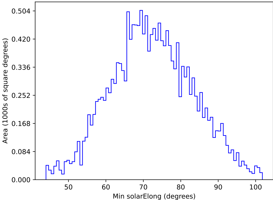
too_elab_heavy_r64_d3_gz_v3.4_10yrs WFD g band: Min solarElong
