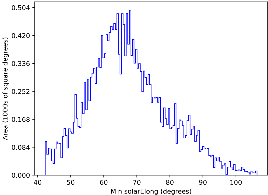
too_elab_heavy_r64_d3_gz_v3.4_10yrs All sky y band: Min solarElong
