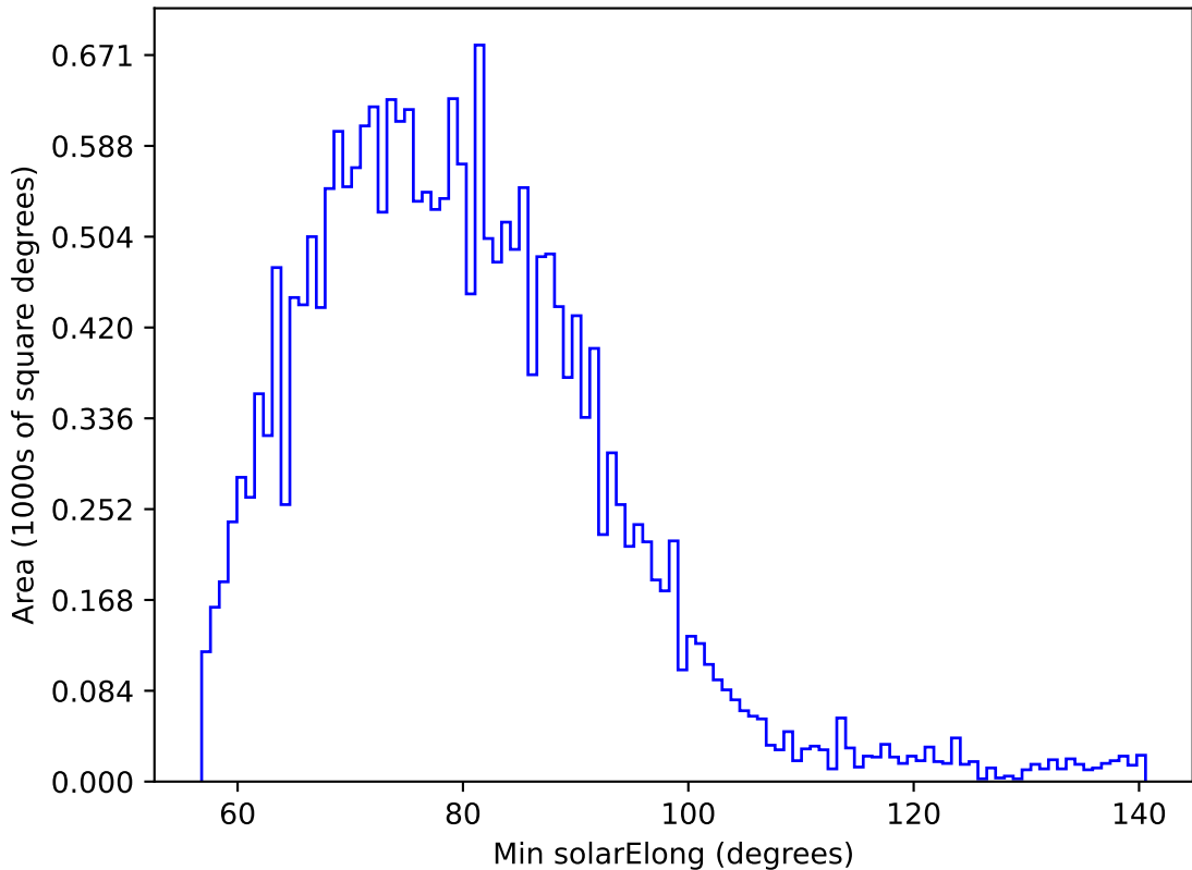
too_elab_heavy_r64_d3_gz_v3.4_10yrs All sky u band: Min solarElong
