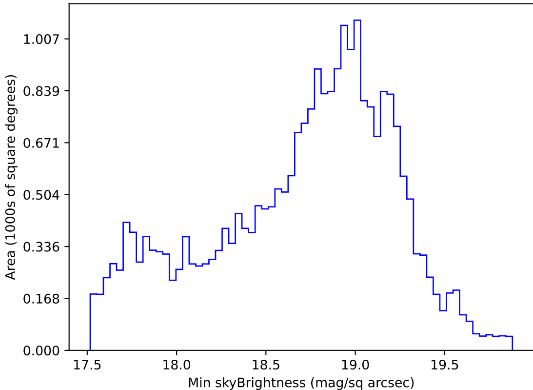
too_elab_heavy_r64_d3_gz_v3.4_10yrs Yr 1 i band: Min skyBrightness
