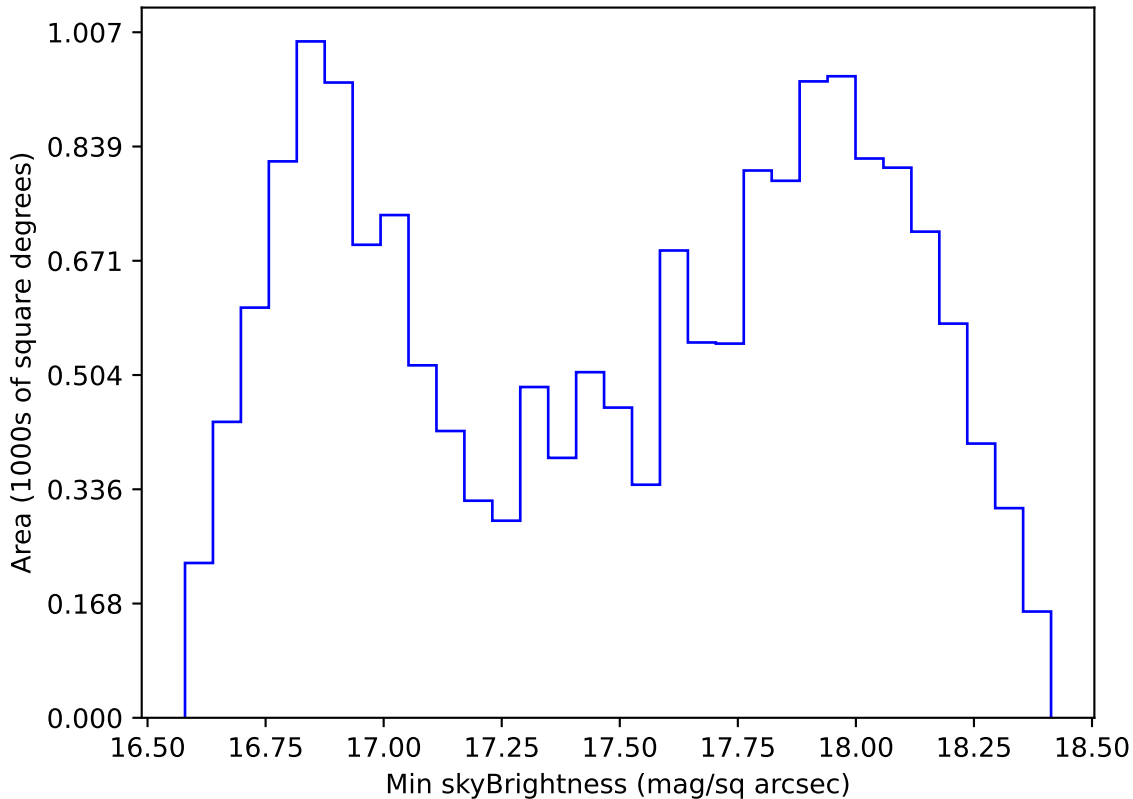
too_elab_heavy_r64_d3_gz_v3.4_10yrs WFD z band: Min skyBrightness
