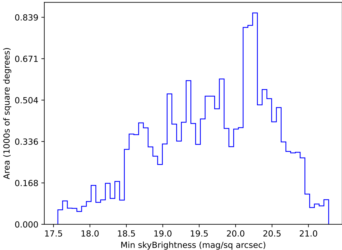
too_elab_heavy_r64_d3_gz_v3.4_10yrs WFD g band: Min skyBrightness
