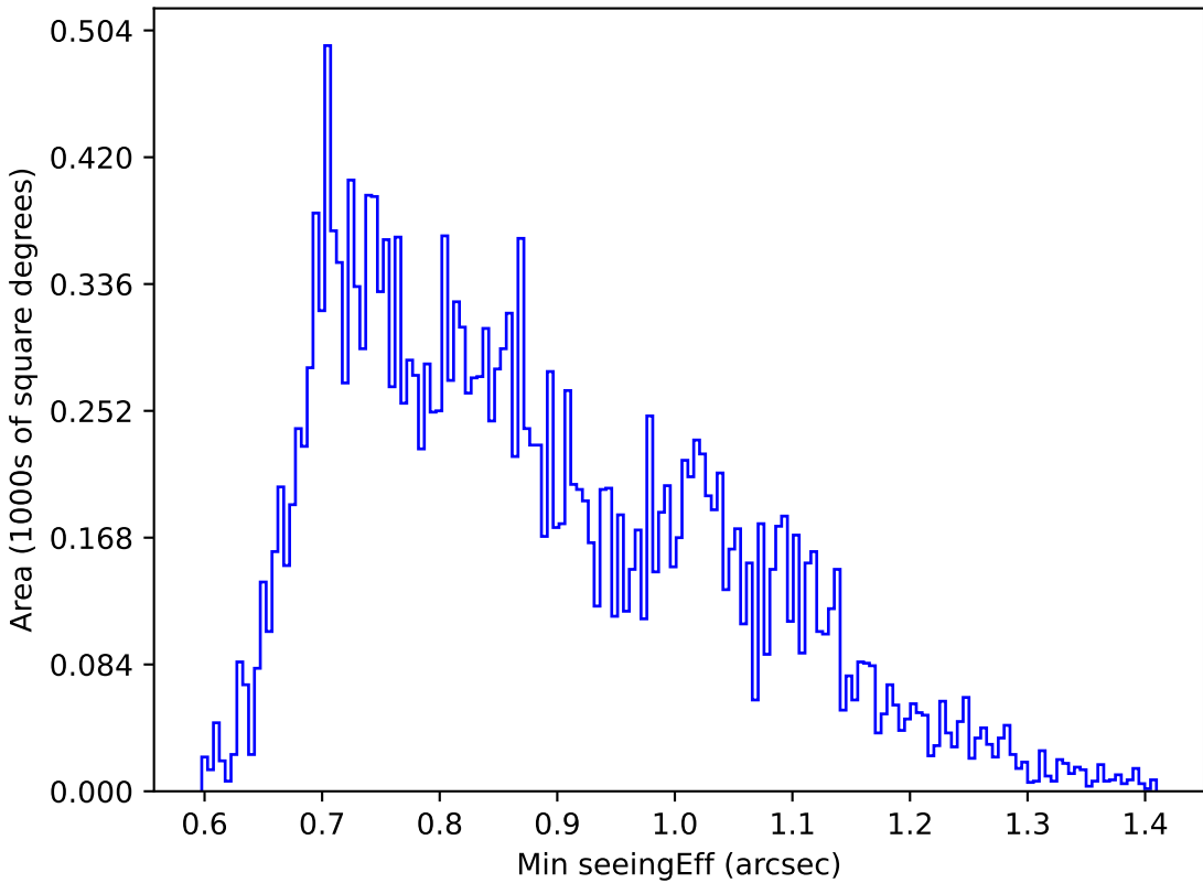
too_elab_heavy_r64_d3_gz_v3.4_10yrs Yr 1 u band: Min seeingEff
