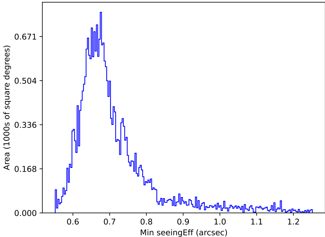
too_elab_heavy_r64_d3_gz_v3.4_10yrs Yr 1 i band: Min seeingEff
