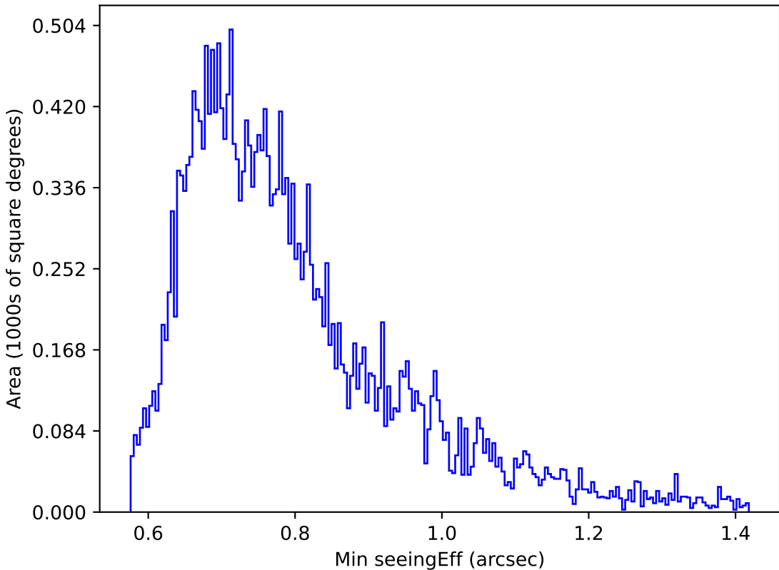
too_elab_heavy_r64_d3_gz_v3.4_10yrs Yr 1 g band: Min seeingEff
