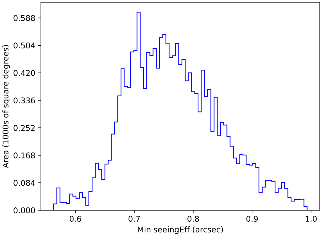
too_elab_heavy_r64_d3_gz_v3.4_10yrs WFD u band: Min seeingEff
